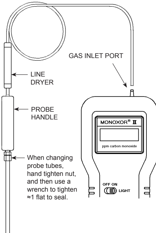
Figure 3. Probe Installation
